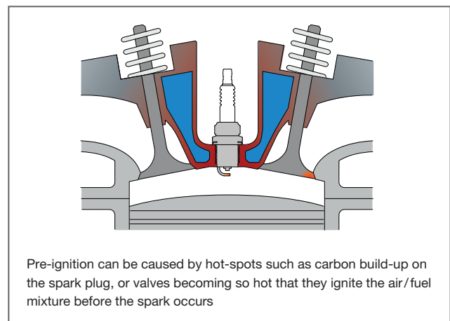
Fig 5.8 Pre-ignition
