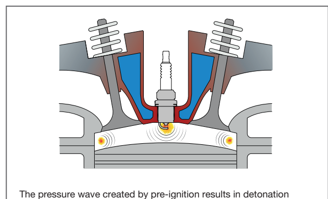
Fig 5.9 Engine knock
